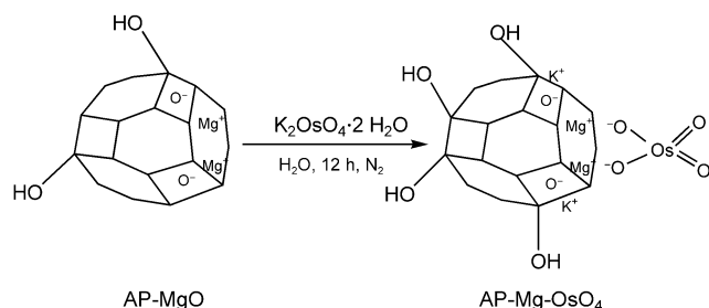
Scheme 1. Preparation of AP-Mg-OsO 4 catalyst.
