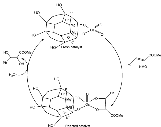
Scheme 2. Proposed mechanism for the AP-Mg-OsO 4 -catalysed dihydroxylation of olefins.
